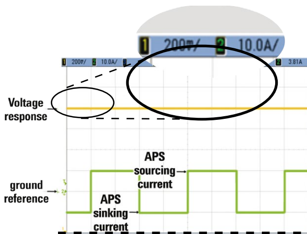
Figure 3 shows an example of an APS power supply smoothly pulsing back and forth from sinking current at -10 A to sourcing current at 10 A. Notice that the voltage level captured at high resolution on the top trace remains constant with no glitches.
