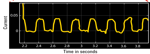
Figure 1. Dynamic current measurement
