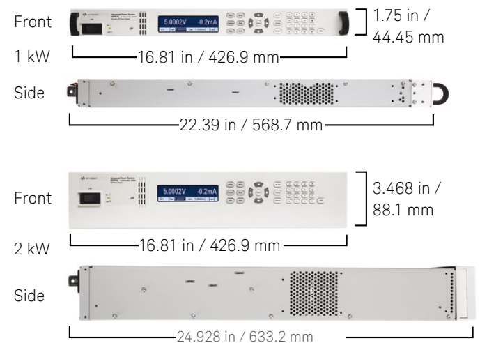
Figure 12. 1 kW and 2 kW power supplies, front and side dimensions
