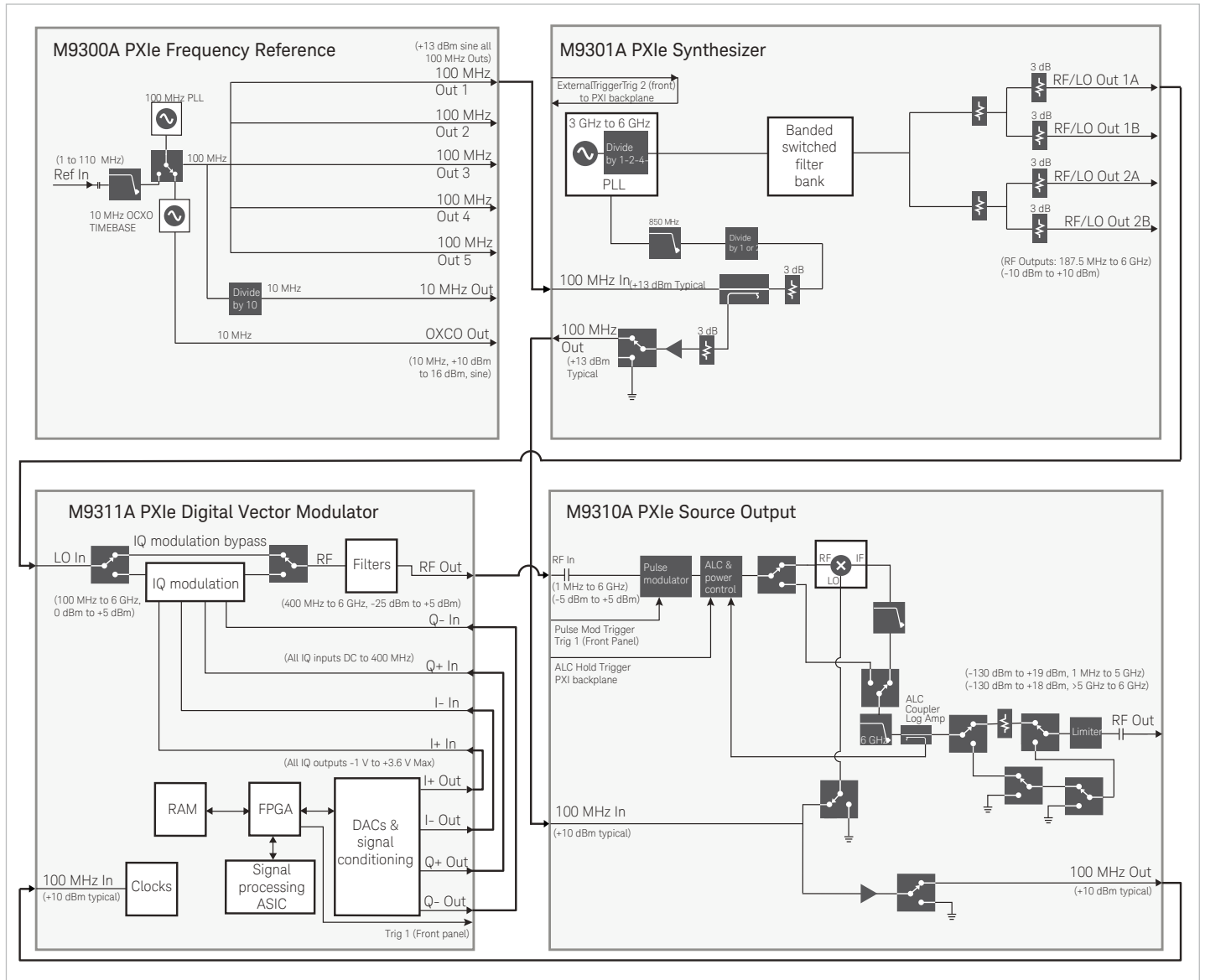
Figure 5. M9381A PXle vector signal generator block diagram with four modules consisting of the M9301A synthesizer, M9310A source output, M9311A digital vector modulator, and optional M9300A frequency reference.
