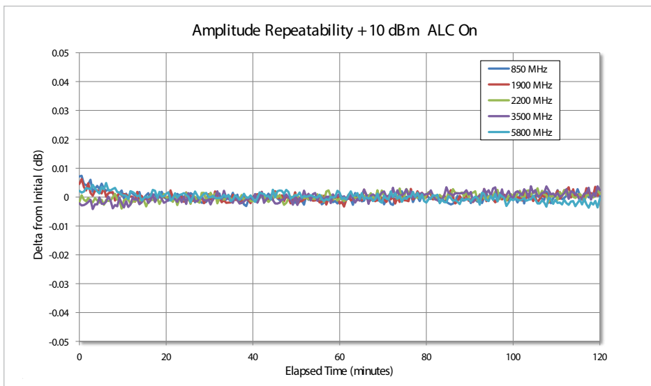
Figure 8. Amplitude repeatability at various carrier frequencies. Repeatability measures the ability of the instrument to return to a given power setting after a random excursion to any other frequency and power setting. It should not be confused with absolute level accuracy.
