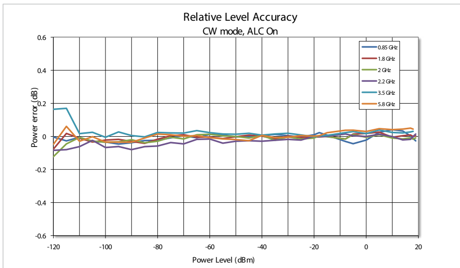
Figure 9. Relative level accuracy at various carrier frequencies.
