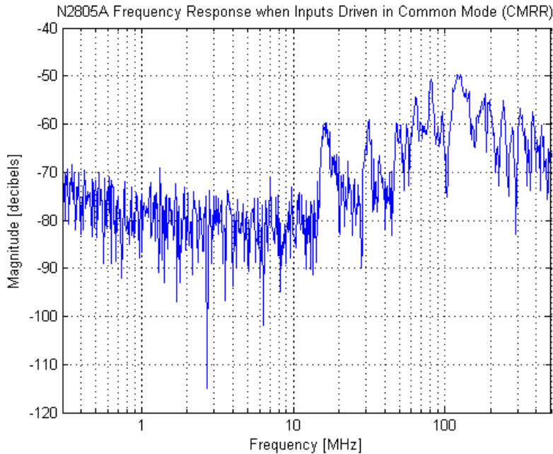
Figure 11. N2805A common mode rejection ratio.
