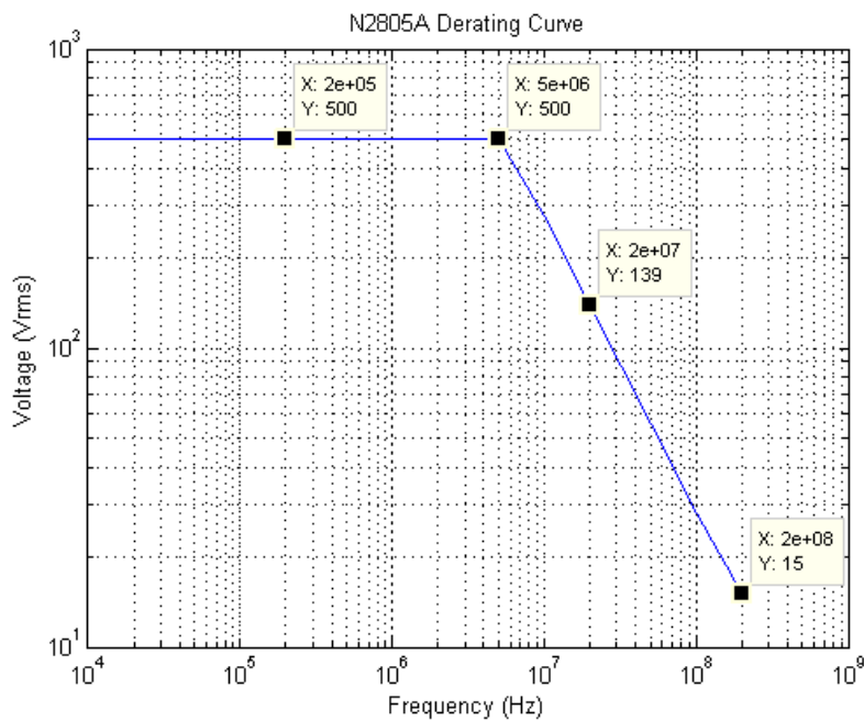
Figure 12. N2805A derating characteristics over frequency.
